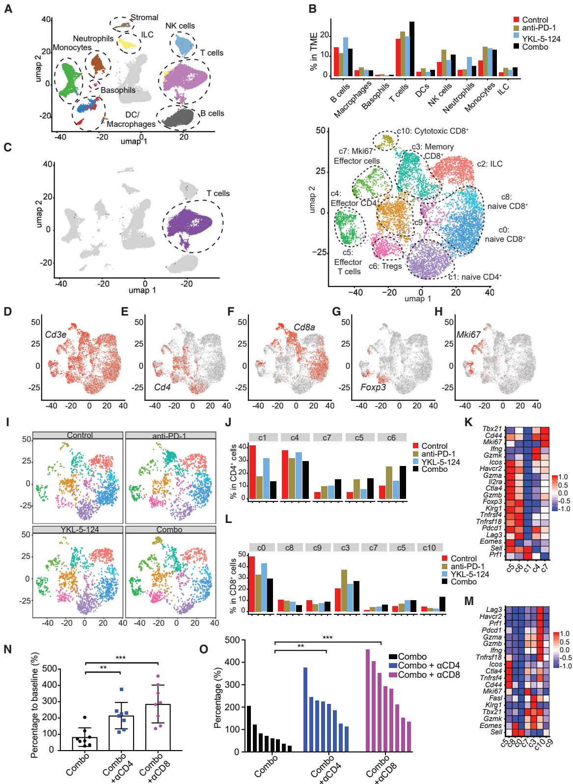
Figure 7. Combinatorial Therapy Reinigorates Anti-tumor Immunity
