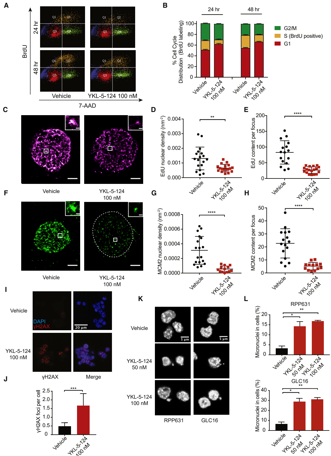
Figure 2. CDK7 Inhibition Impairs DNA Synthesis and MCM2 Complex and Causes DNA Damage and Micronuclei Formation
