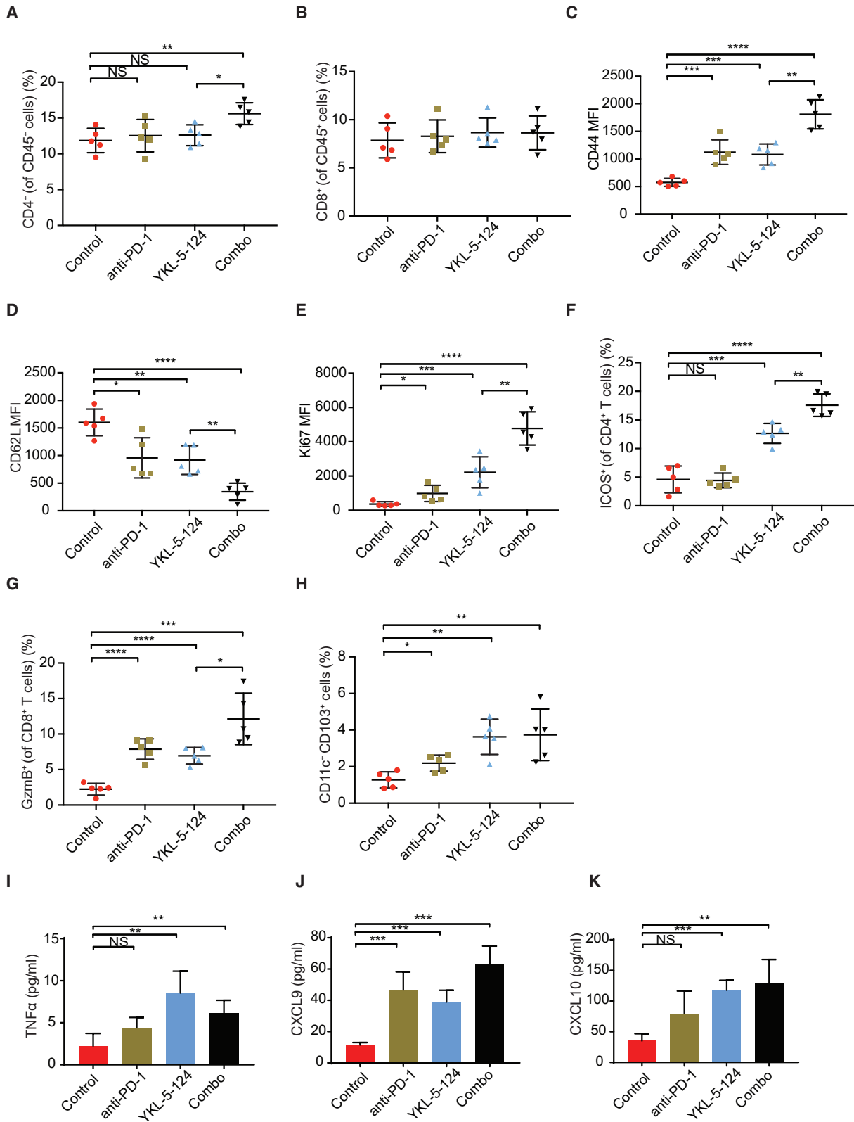
Figure 5. YKL-5-124 Provokes a Robust Anti-tumor Immune Program, Which Is Further Enhanced by Anti-PD-1 Immunotherapy
