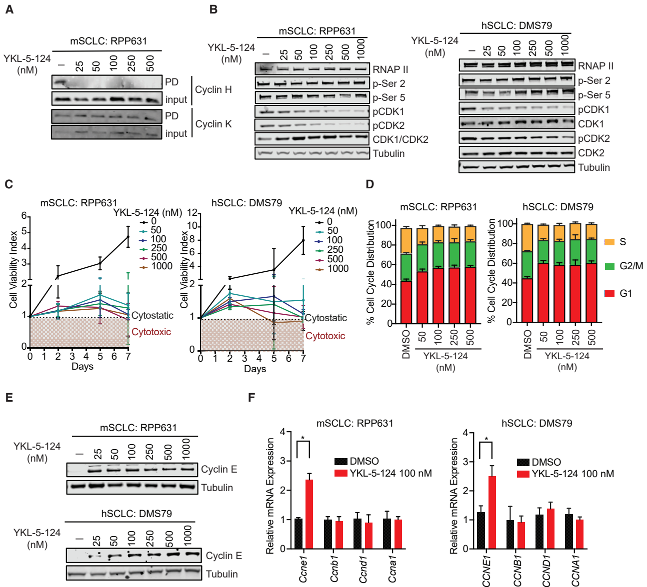
Figure 1. YKL-5-124 Specifically Targets CDK7 and Disrupts Cell-Cycle Progression through Inhibition of CDK7 CAK Activity
